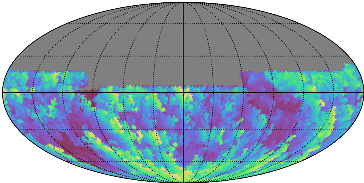
early_u_fpextra3.0_v3.4_10yrs All sky u band: Max airmass
