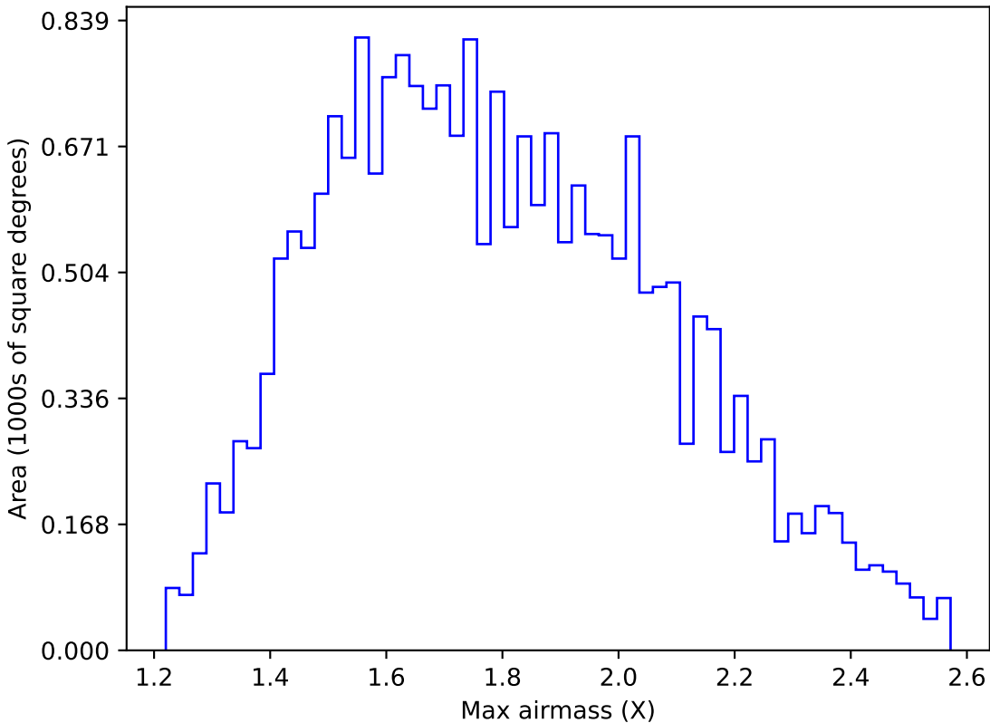
early_u_fpextra3.0_v3.4_10yrs All sky u band: Max airmass
