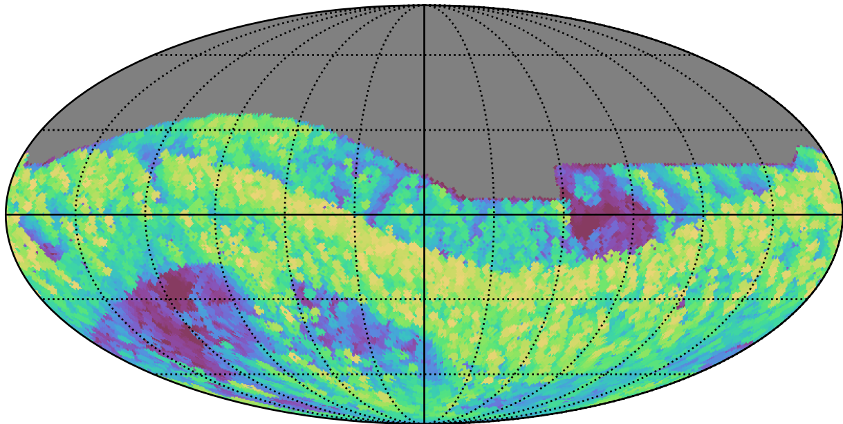
early_u_fpextra3.0_v3.4_10yrs All sky i band: Max airmass
