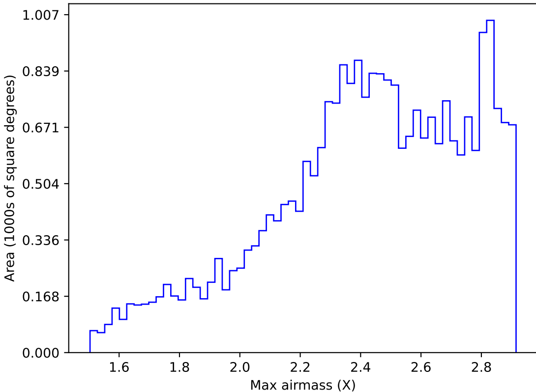
early_u_fpextra3.0_v3.4_10yrs All sky i band: Max airmass
