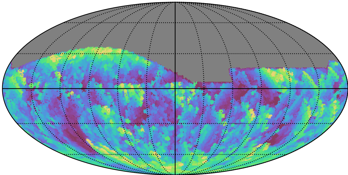
early_u_fpextra3.0_v3.4_10yrs All sky g band: Max airmass
