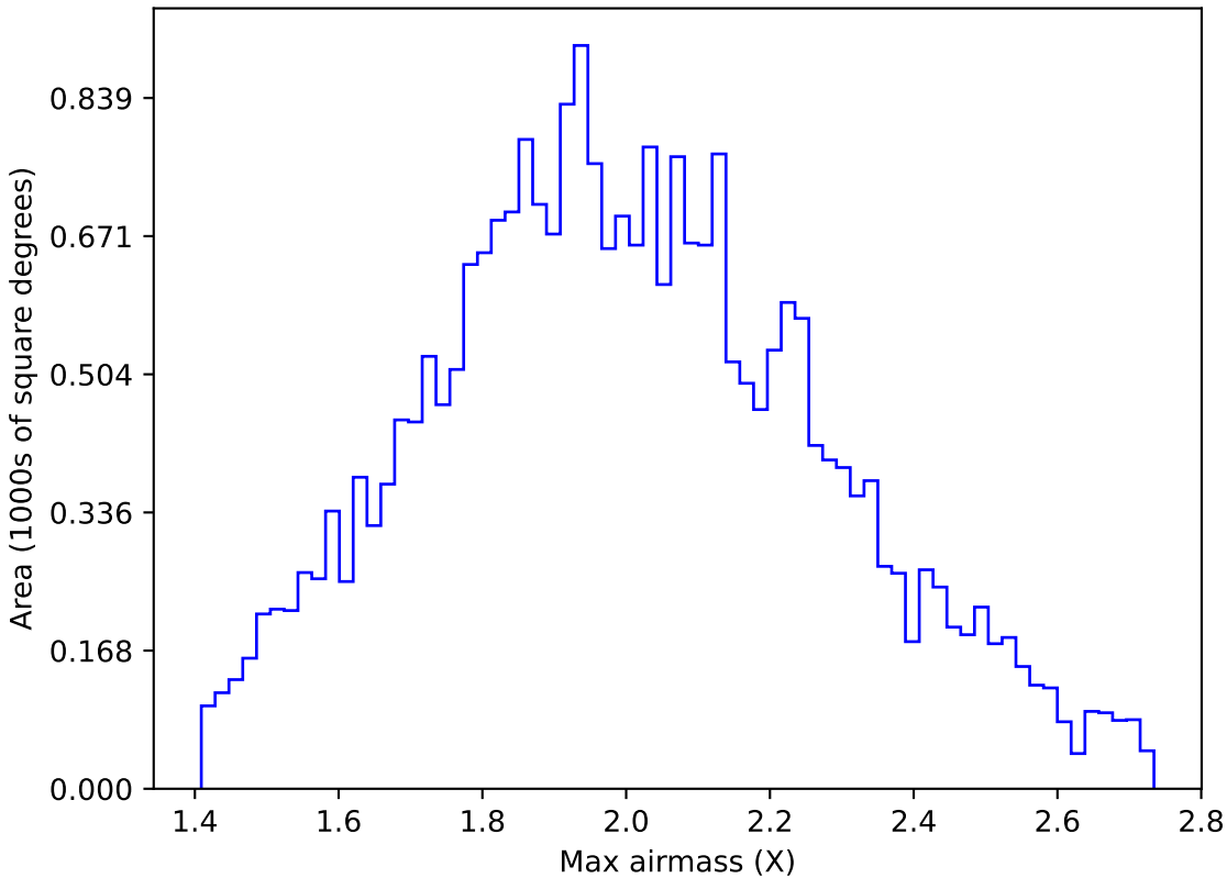
early_u_fpextra3.0_v3.4_10yrs All sky g band: Max airmass
