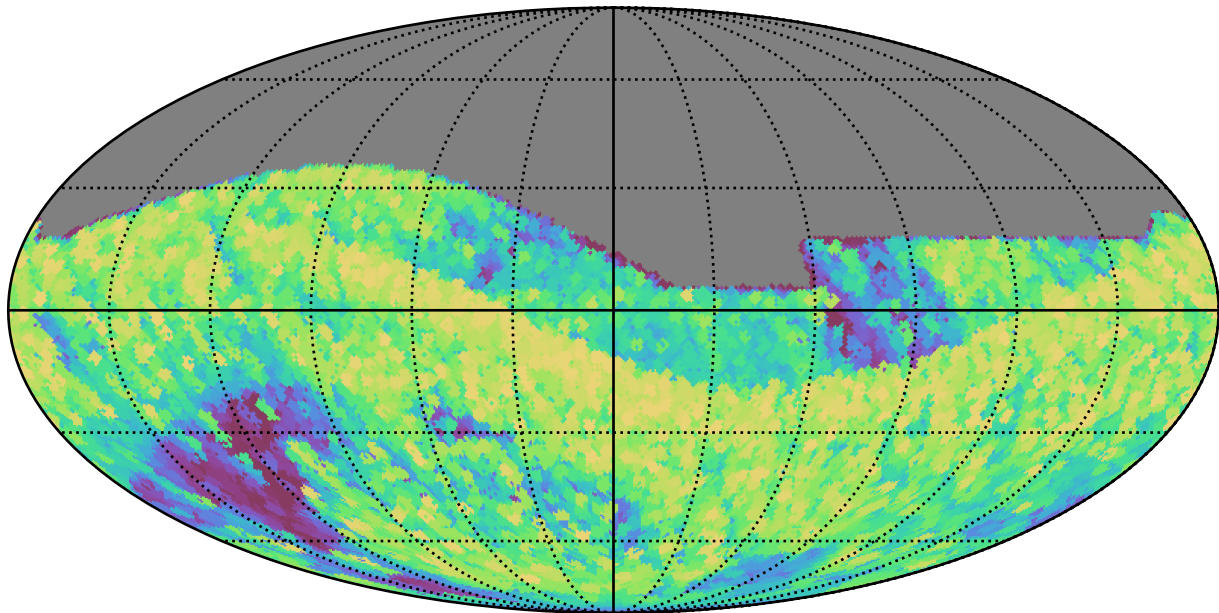
early_u_fpextra3.0_v3.4_10yrs All sky all bands: Max airmass
