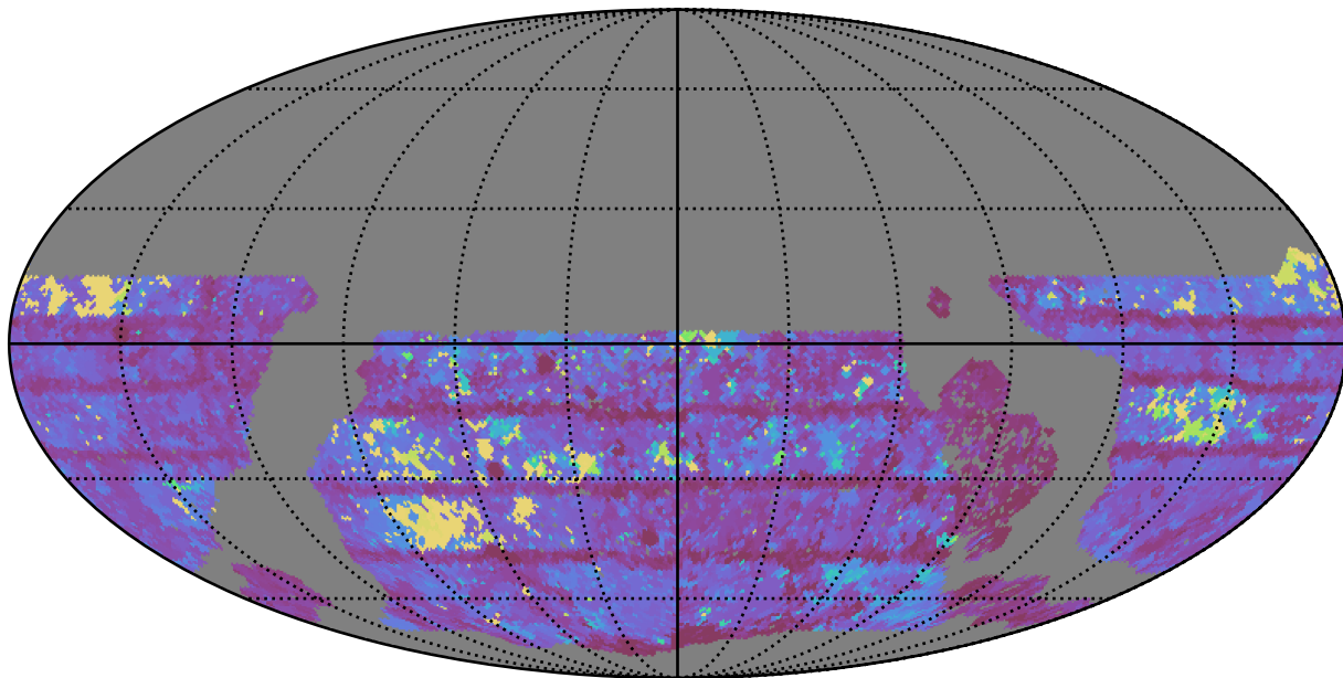
early_u_fpextra3.0_v3.4_10yrs WFD z band: Max Inter-Night Gap
