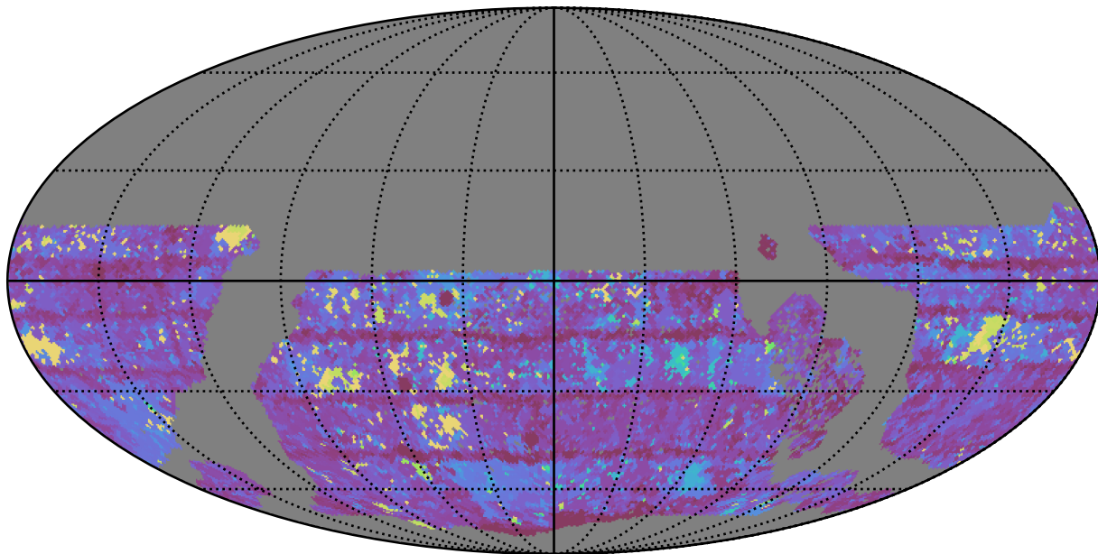
early_u_fpextra3.0_v3.4_10yrs WFD y band: Max Inter-Night Gap
