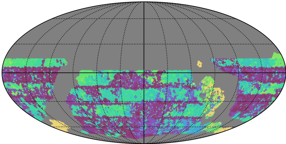
early_u_fpextra3.0_v3.4_10yrs WFD u band: Max Inter-Night Gap
