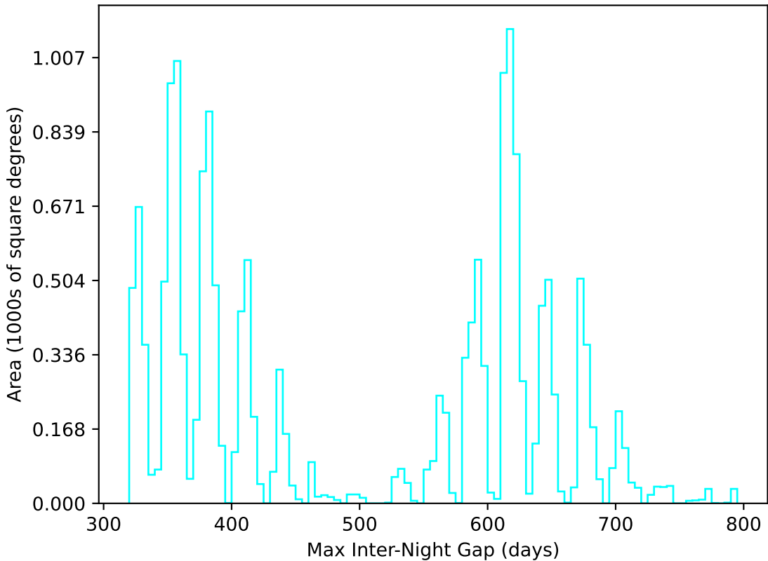
early_u_fpextra3.0_v3.4_10yrs WFD u band: Max Inter-Night Gap
