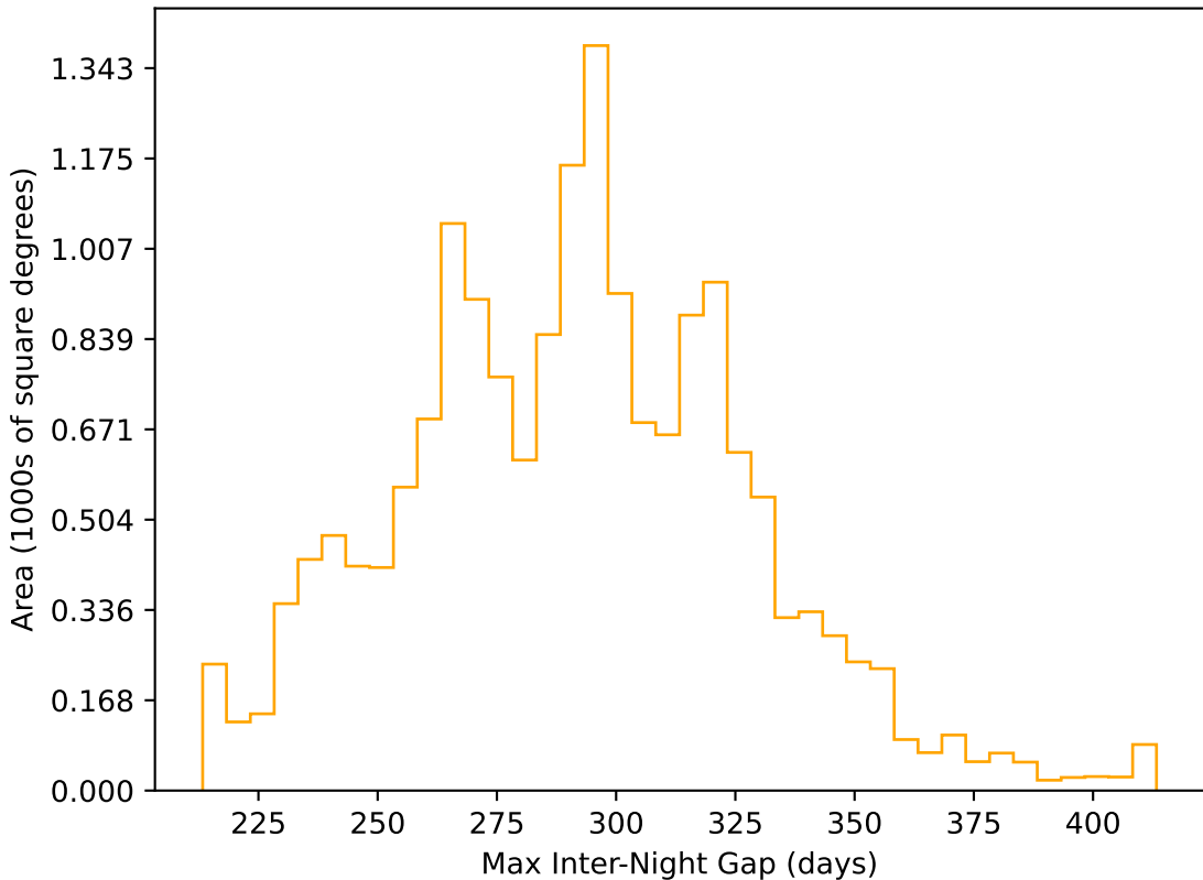
early_u_fpextra3.0_v3.4_10yrs WFD r band: Max Inter-Night Gap
