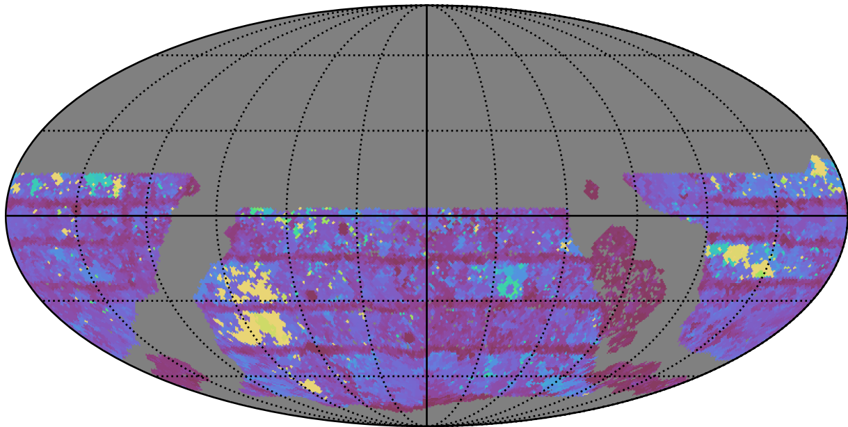
early_u_fpextra3.0_v3.4_10yrs WFD i band: Max Inter-Night Gap
