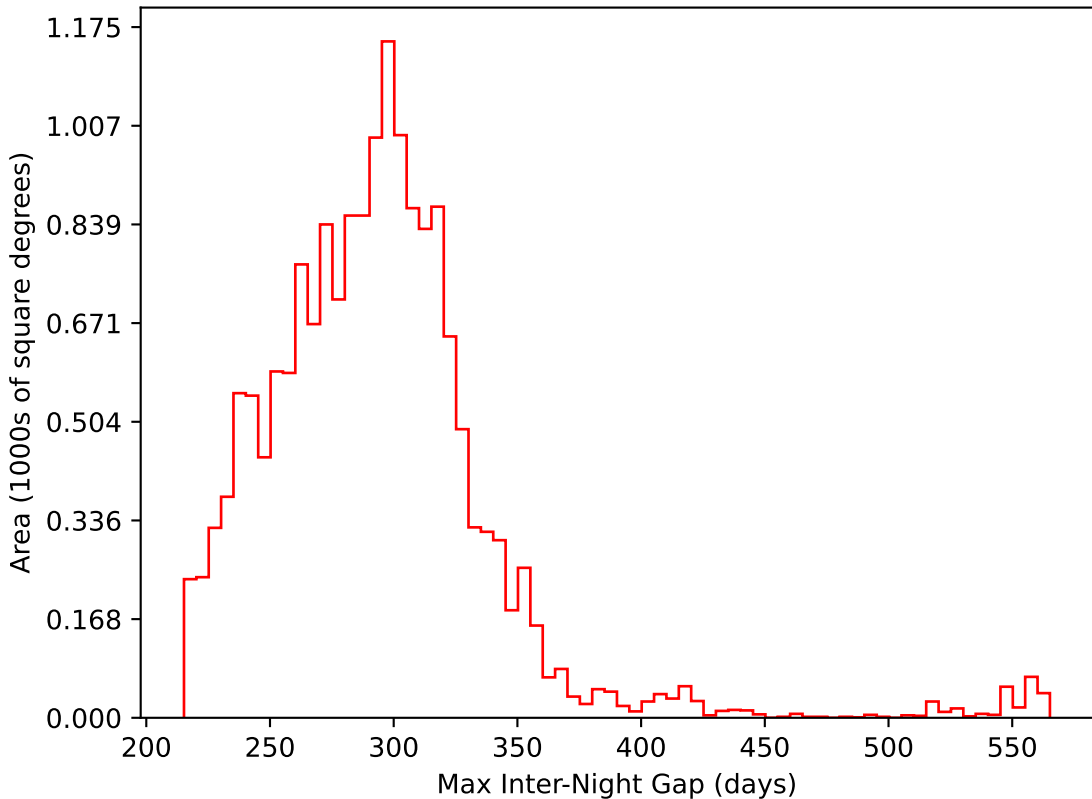
early_u_fpextra3.0_v3.4_10yrs WFD i band: Max Inter-Night Gap
