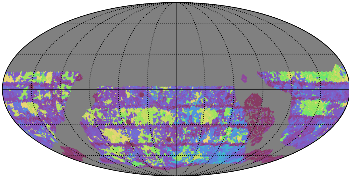
early_u_fpextra3.0_v3.4_10yrs WFD g band: Max Inter-Night Gap
