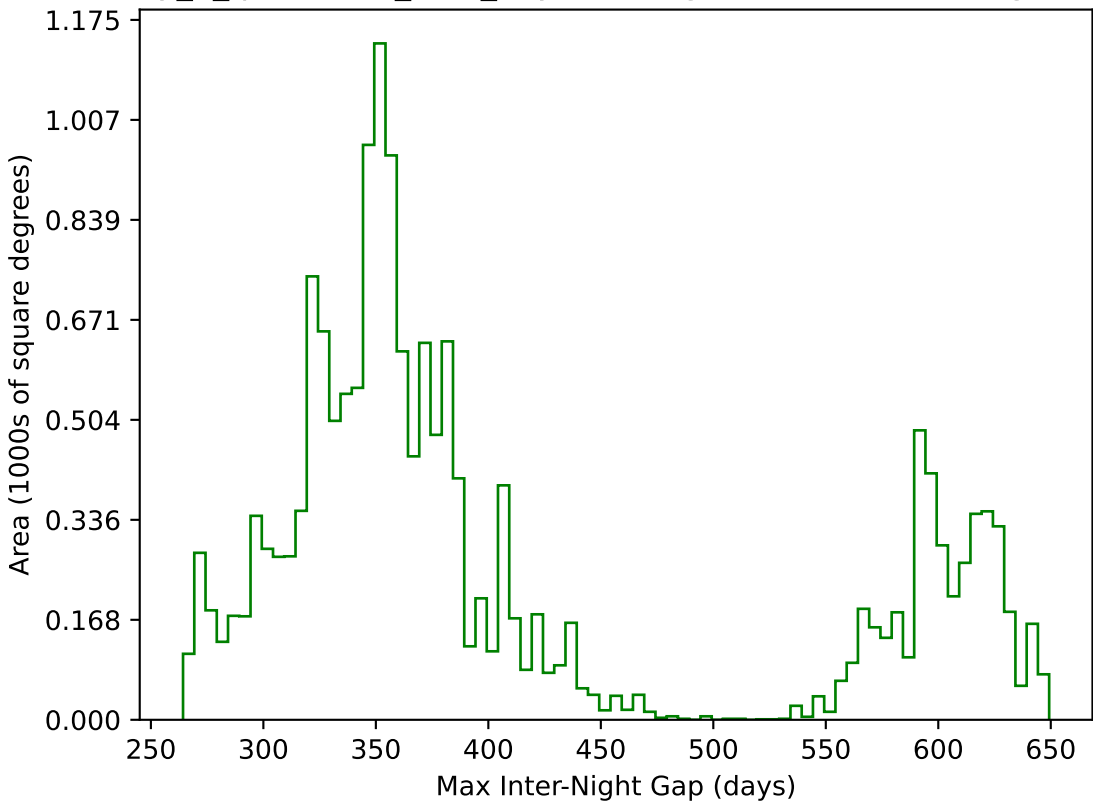
early_u_fpextra3.0_v3.4_10yrs WFD g band: Max Inter-Night Gap
