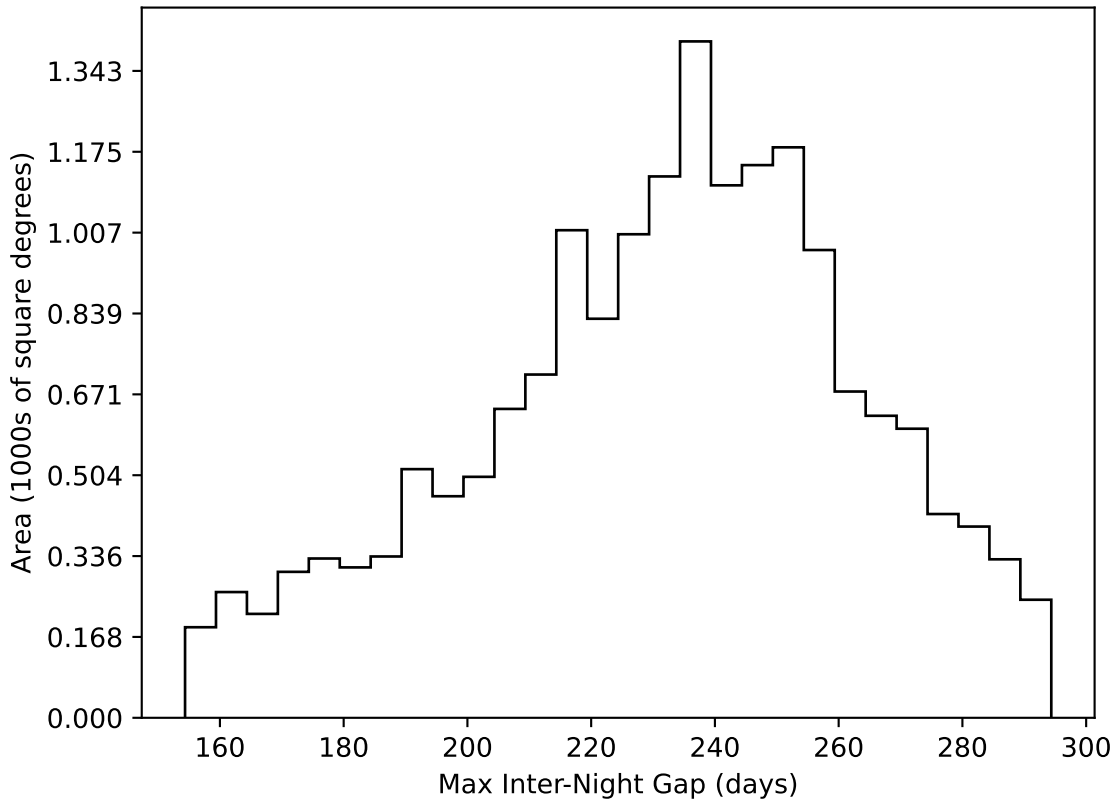
early_u_fpextra3.0_v3.4_10yrs WFD all bands: Max Inter-Night Gap
