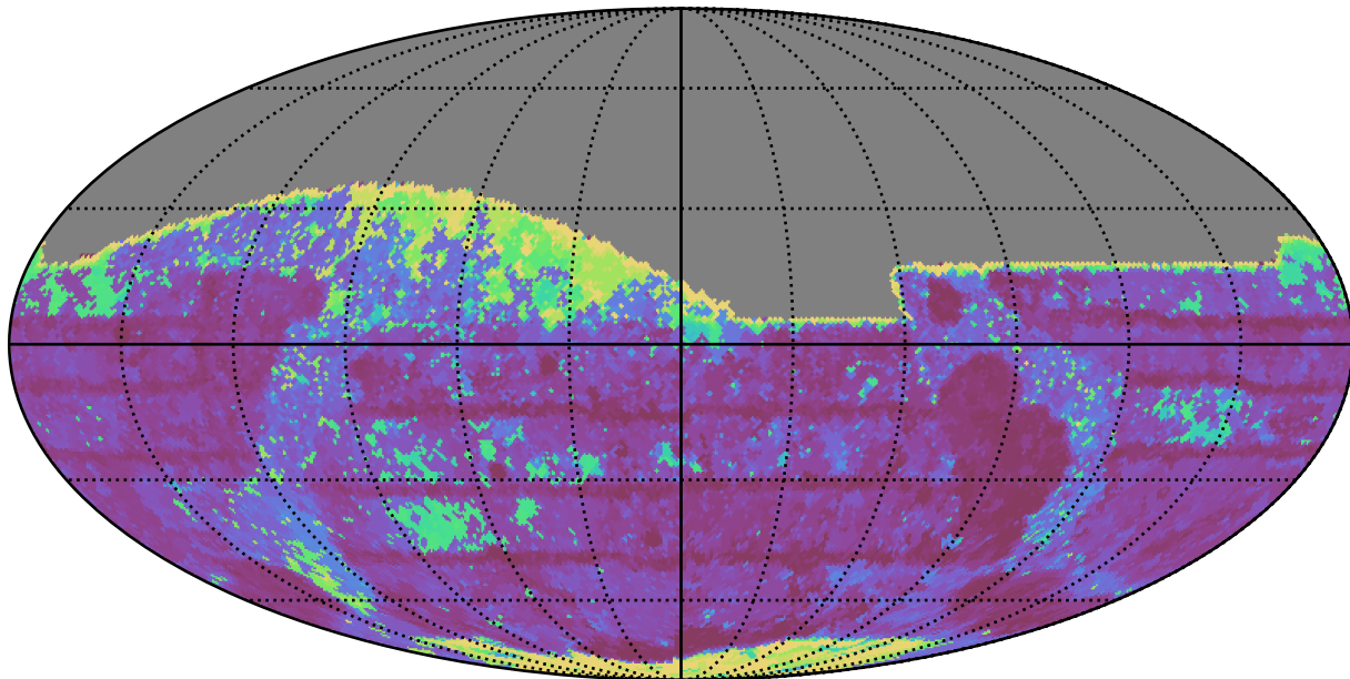
early_u_fpextra3.0_v3.4_10yrs All sky z band: Max Inter-Night Gap
