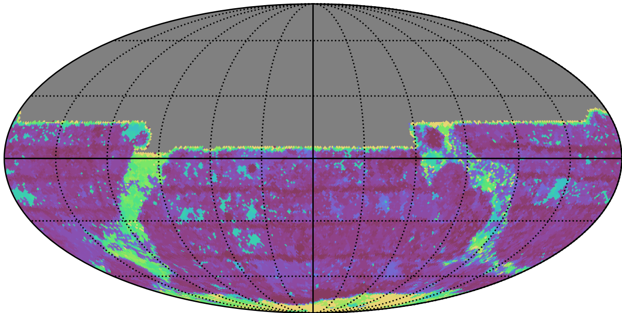
early_u_fpextra3.0_v3.4_10yrs All sky y band: Max Inter-Night Gap
