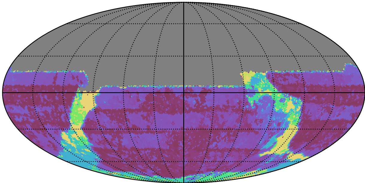
early_u_fpextra3.0_v3.4_10yrs All sky u band: Max Inter-Night Gap
