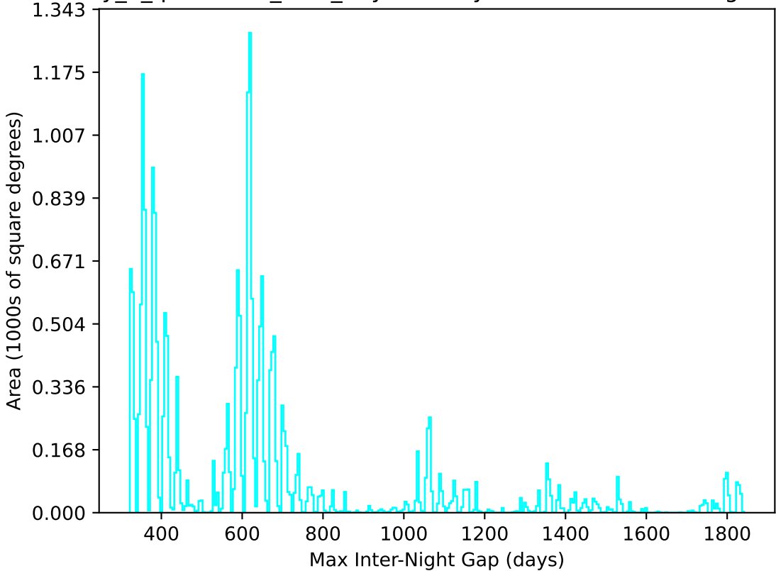
early_u_fpextra3.0_v3.4_10yrs All sky u band: Max Inter-Night Gap
