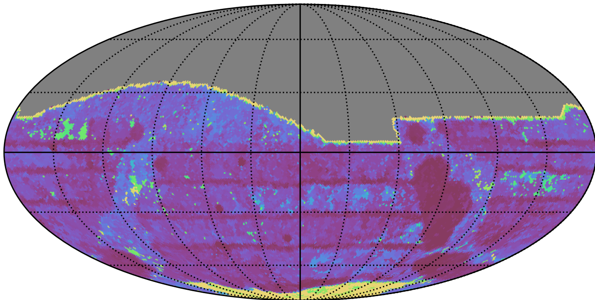
early_u_fpextra3.0_v3.4_10yrs All sky r band: Max Inter-Night Gap
