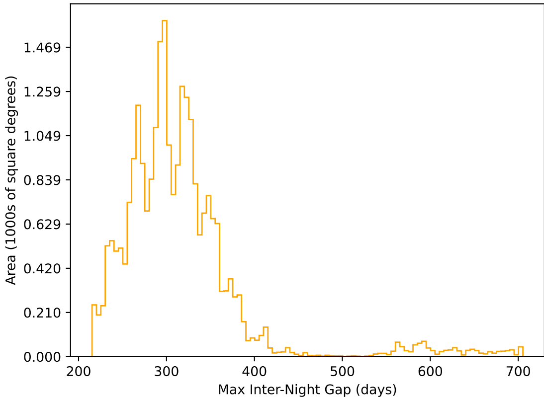
early_u_fpextra3.0_v3.4_10yrs All sky r band: Max Inter-Night Gap
