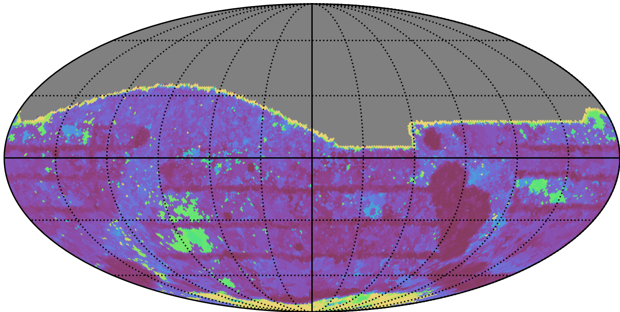
early_u_fpextra3.0_v3.4_10yrs All sky i band: Max Inter-Night Gap
