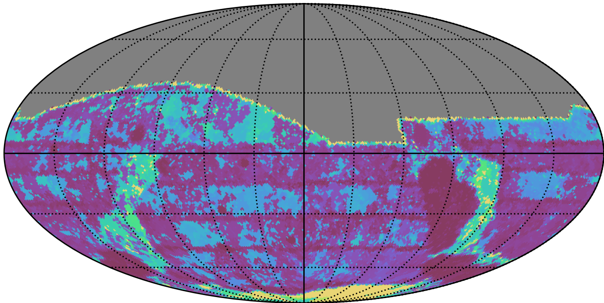
early_u_fpextra3.0_v3.4_10yrs All sky g band: Max Inter-Night Gap
