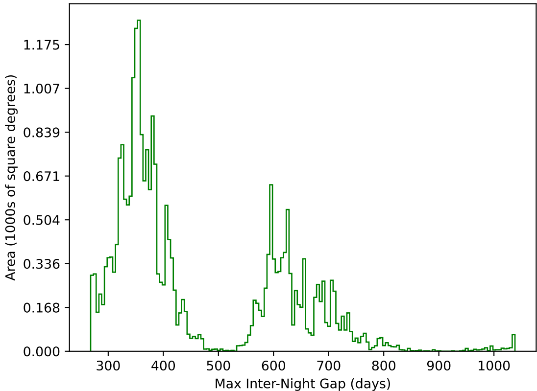
early_u_fpextra3.0_v3.4_10yrs All sky g band: Max Inter-Night Gap
