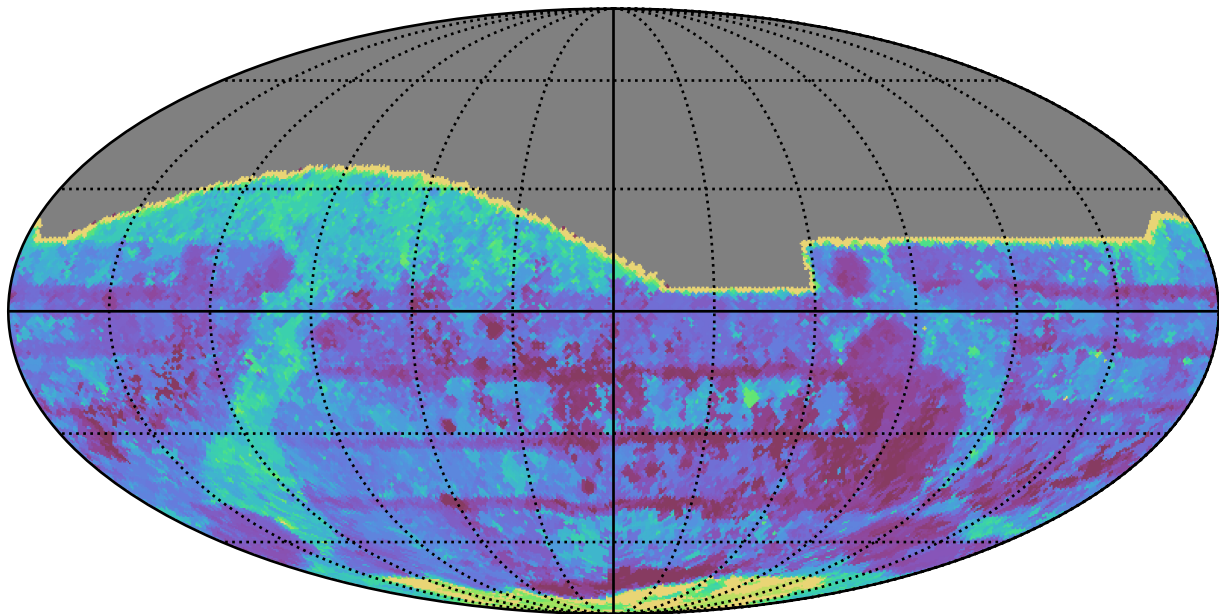
early_u_fpextra3.0_v3.4_10yrs All sky all bands: Max Inter-Night Gap
