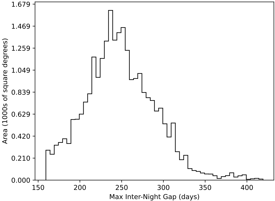
early_u_fpextra3.0_v3.4_10yrs All sky all bands: Max Inter-Night Gap
