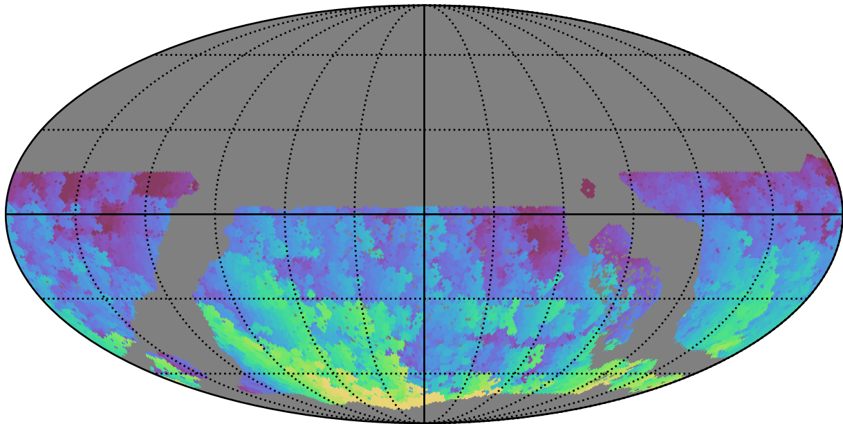
early_u_fpextra3.0_v3.4_10yrs WFD u band: Max HA
