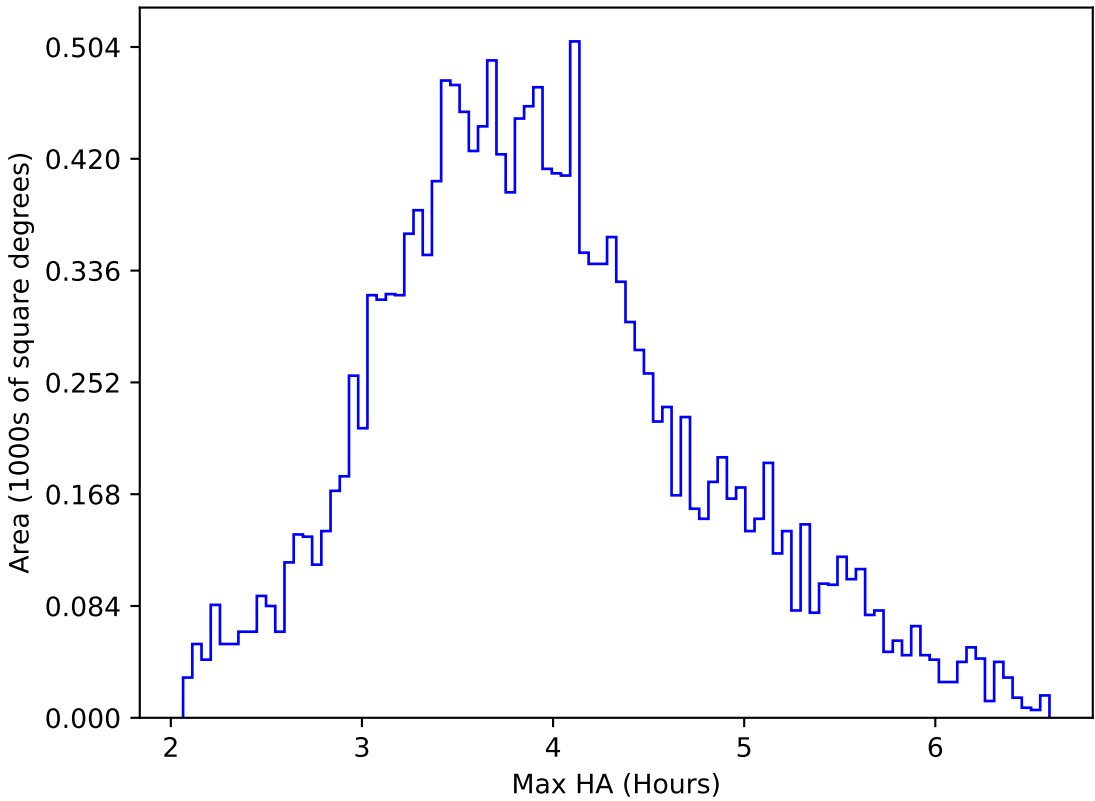
early_u_fpextra3.0_v3.4_10yrs WFD u band: Max HA
