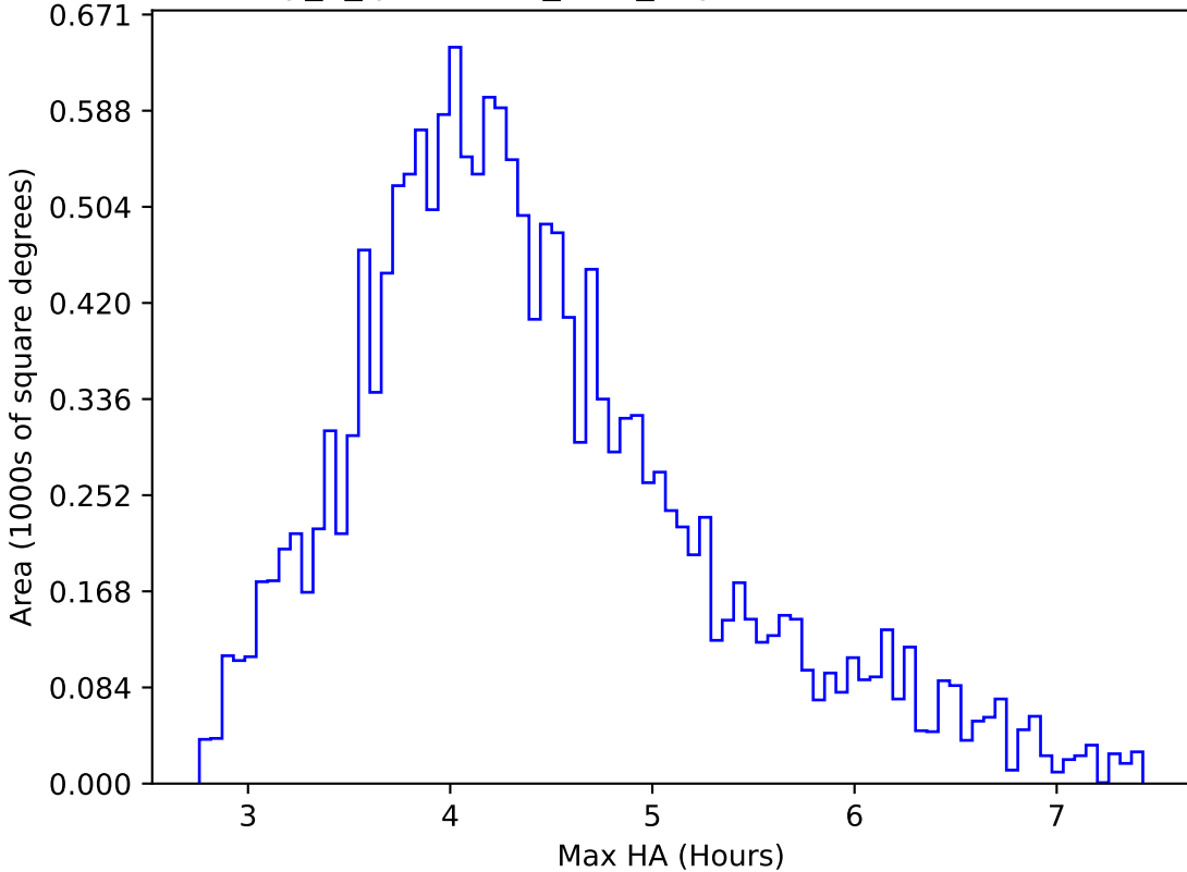
early_u_fpextra3.0_v3.4_10yrs WFD r band: Max HA
