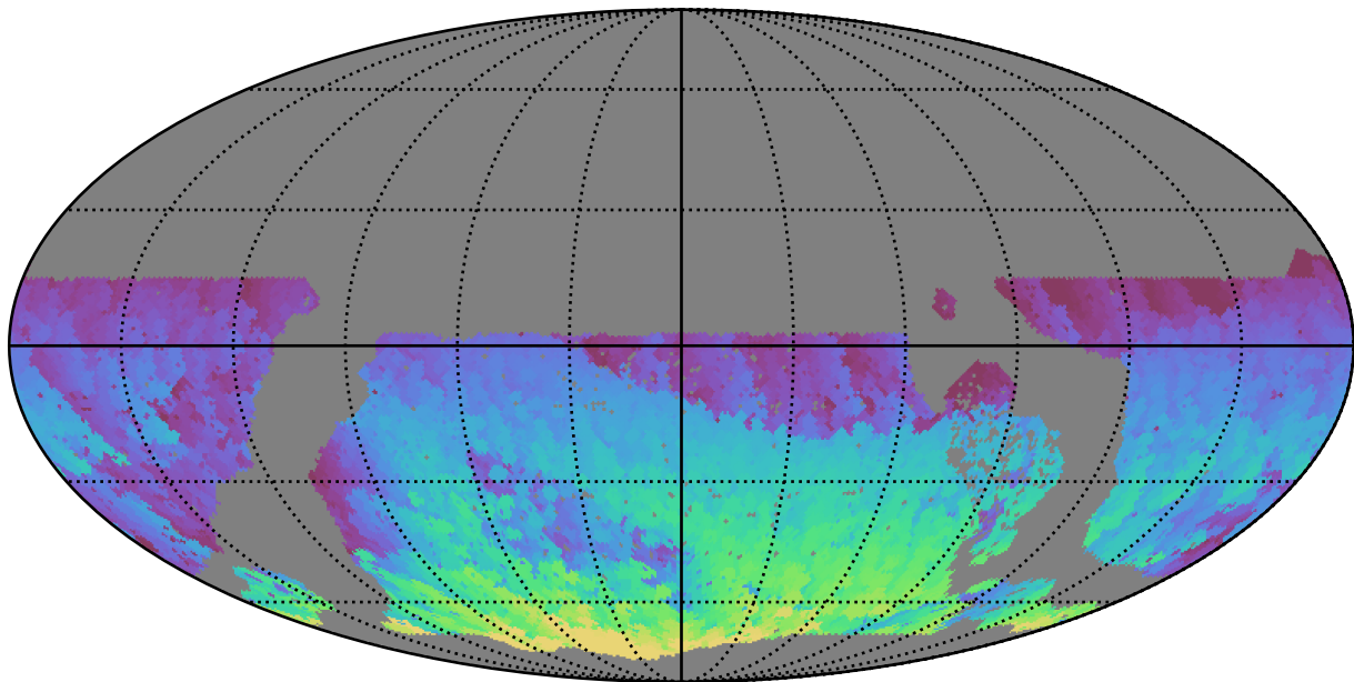
early_u_fpextra3.0_v3.4_10yrs WFD i band: Max HA
