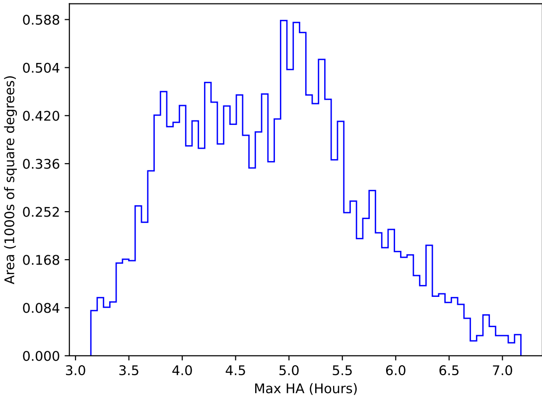
early_u_fpextra3.0_v3.4_10yrs WFD i band: Max HA
