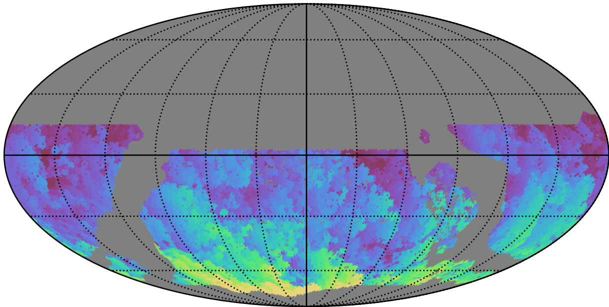
early_u_fpextra3.0_v3.4_10yrs WFD g band: Max HA
