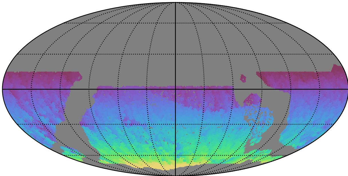
early_u_fpextra3.0_v3.4_10yrs WFD all bands: Max HA
