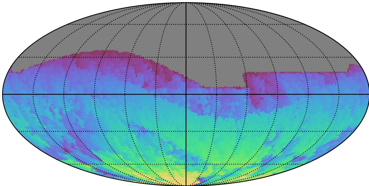
early_u_fpextra3.0_v3.4_10yrs All sky z band: Max HA
