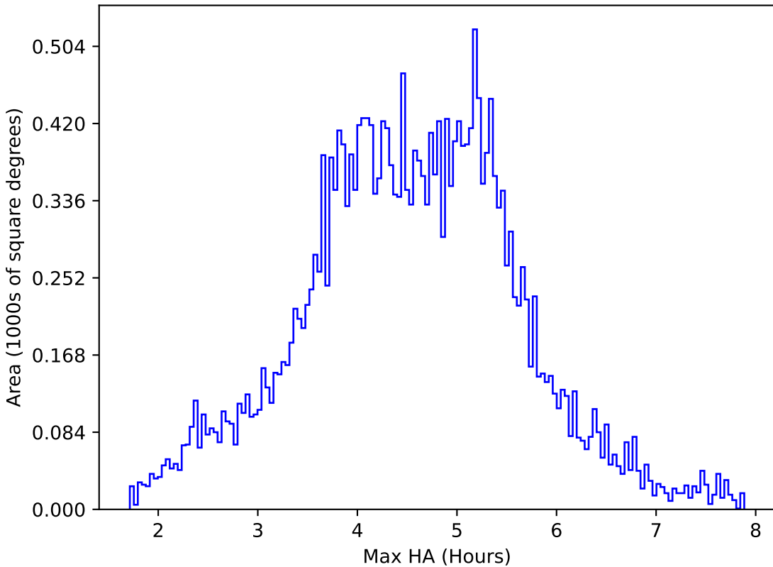
early_u_fpextra3.0_v3.4_10yrs All sky z band: Max HA
