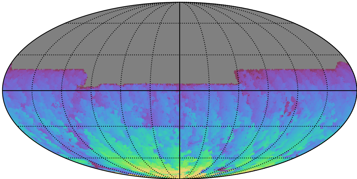
early_u_fpextra3.0_v3.4_10yrs All sky y band: Max HA
