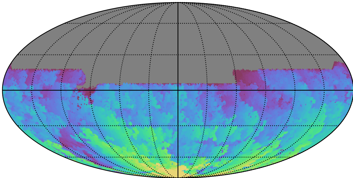
early_u_fpextra3.0_v3.4_10yrs All sky u band: Max HA
