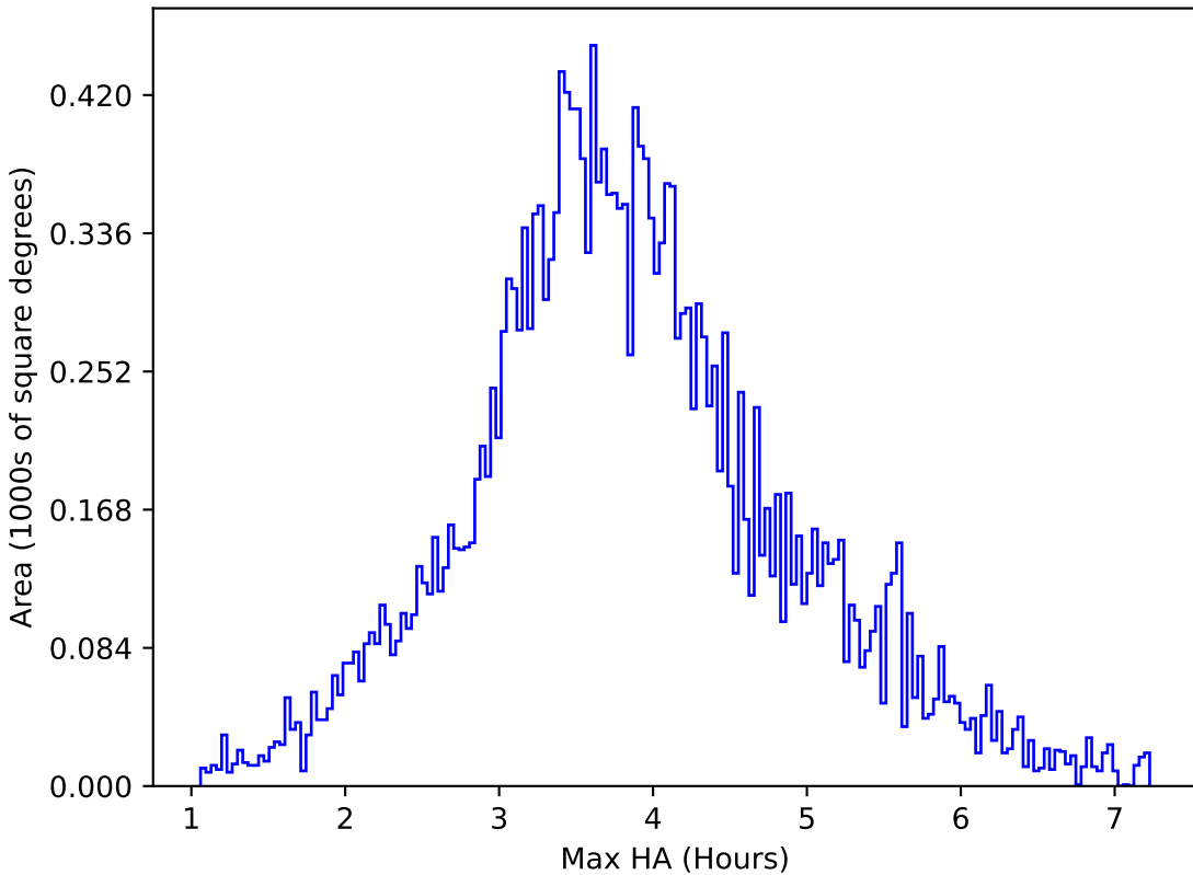
early_u_fpextra3.0_v3.4_10yrs All sky u band: Max HA
