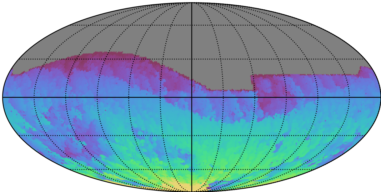
early_u_fpextra3.0_v3.4_10yrs All sky i band: Max HA
