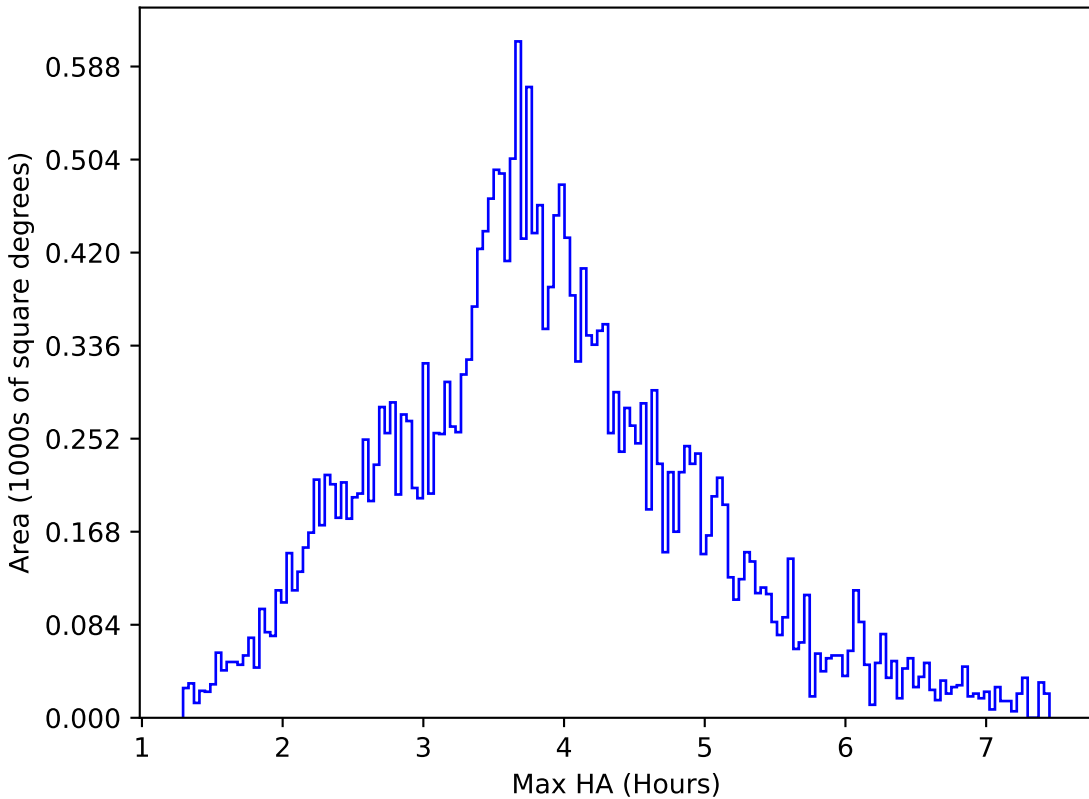
early_u_fpextra3.0_v3.4_10yrs All sky g band: Max HA
