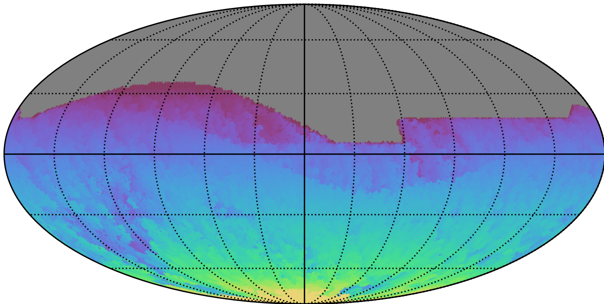
early_u_fpextra3.0_v3.4_10yrs All sky all bands: Max HA
