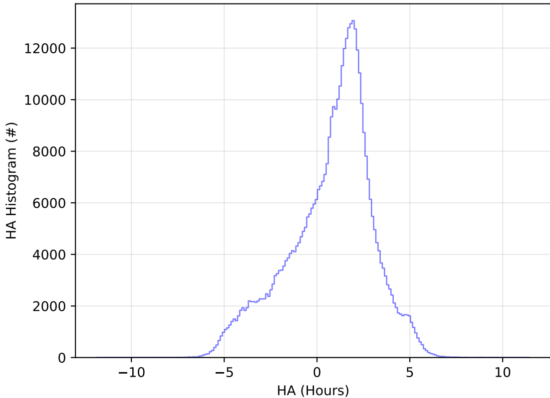
early_u_fpextra3.0_v3.4_10yrs WFD z band: HA Histogram
