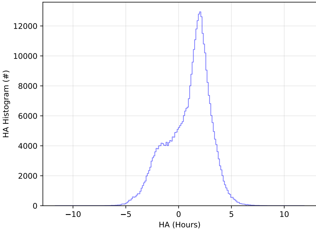
early_u_fpextra3.0_v3.4_10yrs WFD y band: HA Histogram
