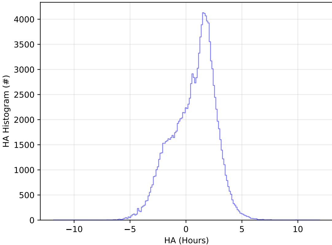
early_u_fpextra3.0_v3.4_10yrs WFD u band: HA Histogram
