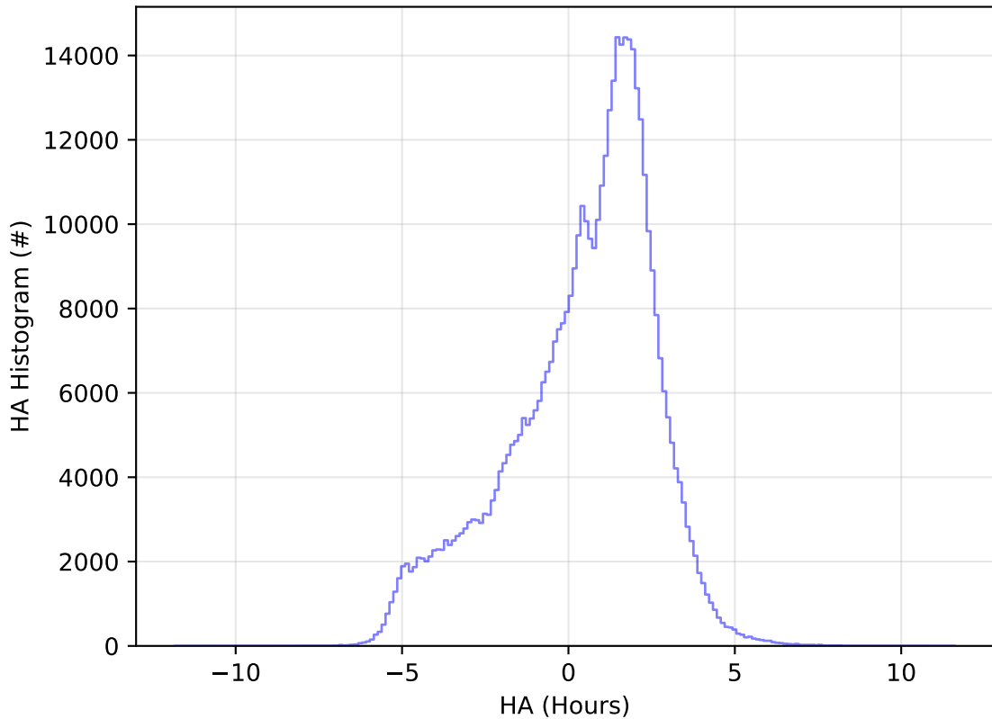
early_u_fpextra3.0_v3.4_10yrs WFD r band: HA Histogram
