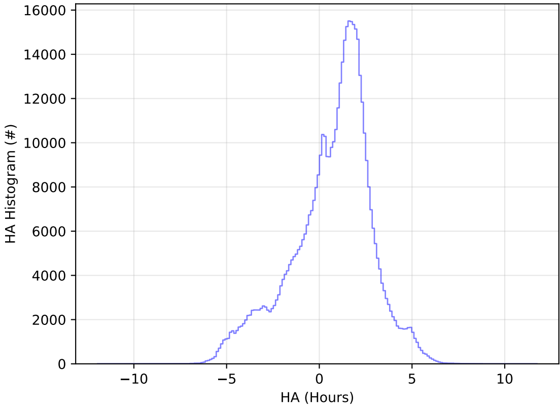
early_u_fpextra3.0_v3.4_10yrs WFD i band: HA Histogram
