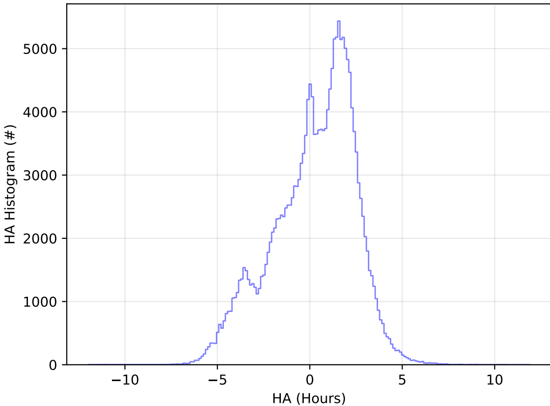
early_u_fpextra3.0_v3.4_10yrs WFD g band: HA Histogram
