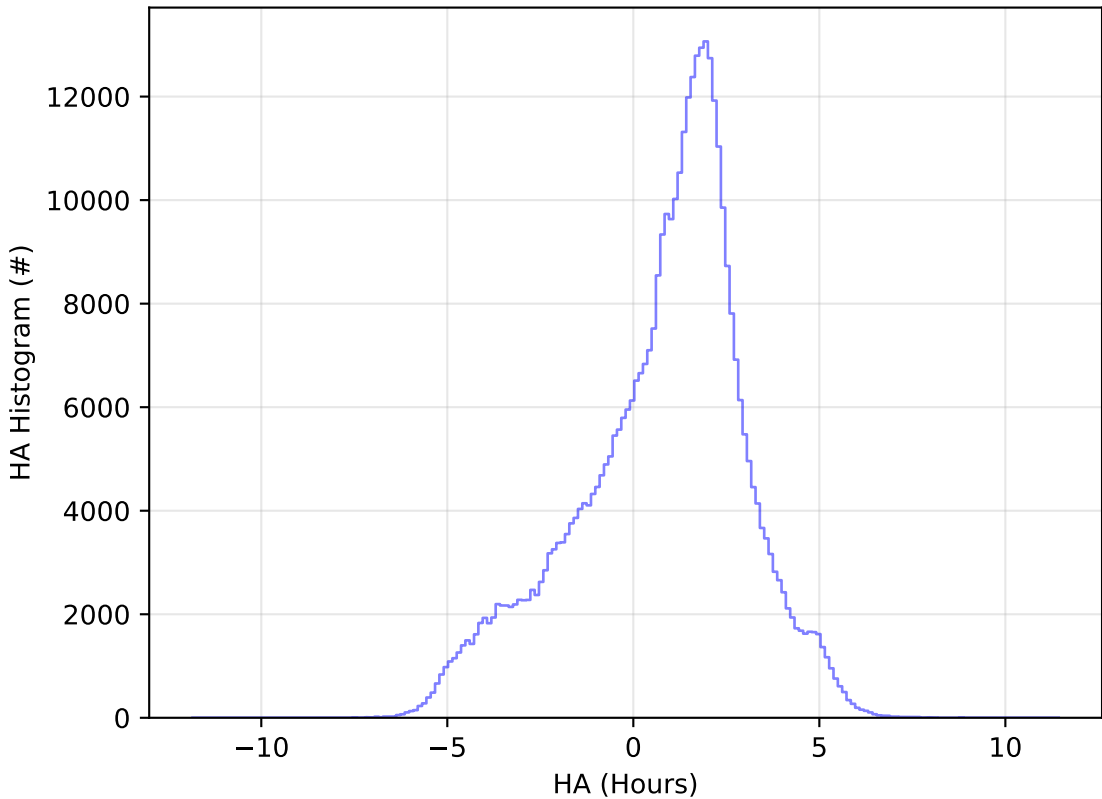
early_u_fpextra3.0_v3.4_10yrs All sky z band: HA Histogram
